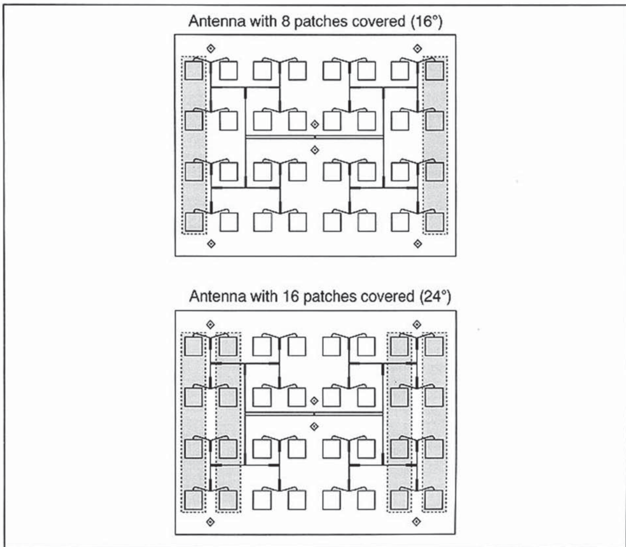
Figure 13. Antenna Configurations
