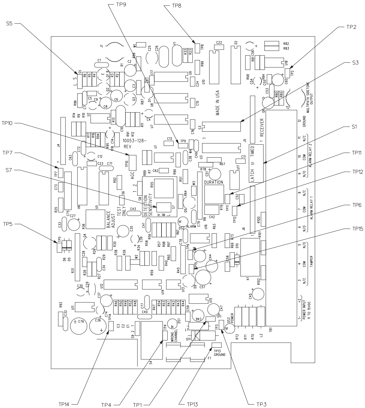
Figure 17. Receiver Circuit Board Component Location
