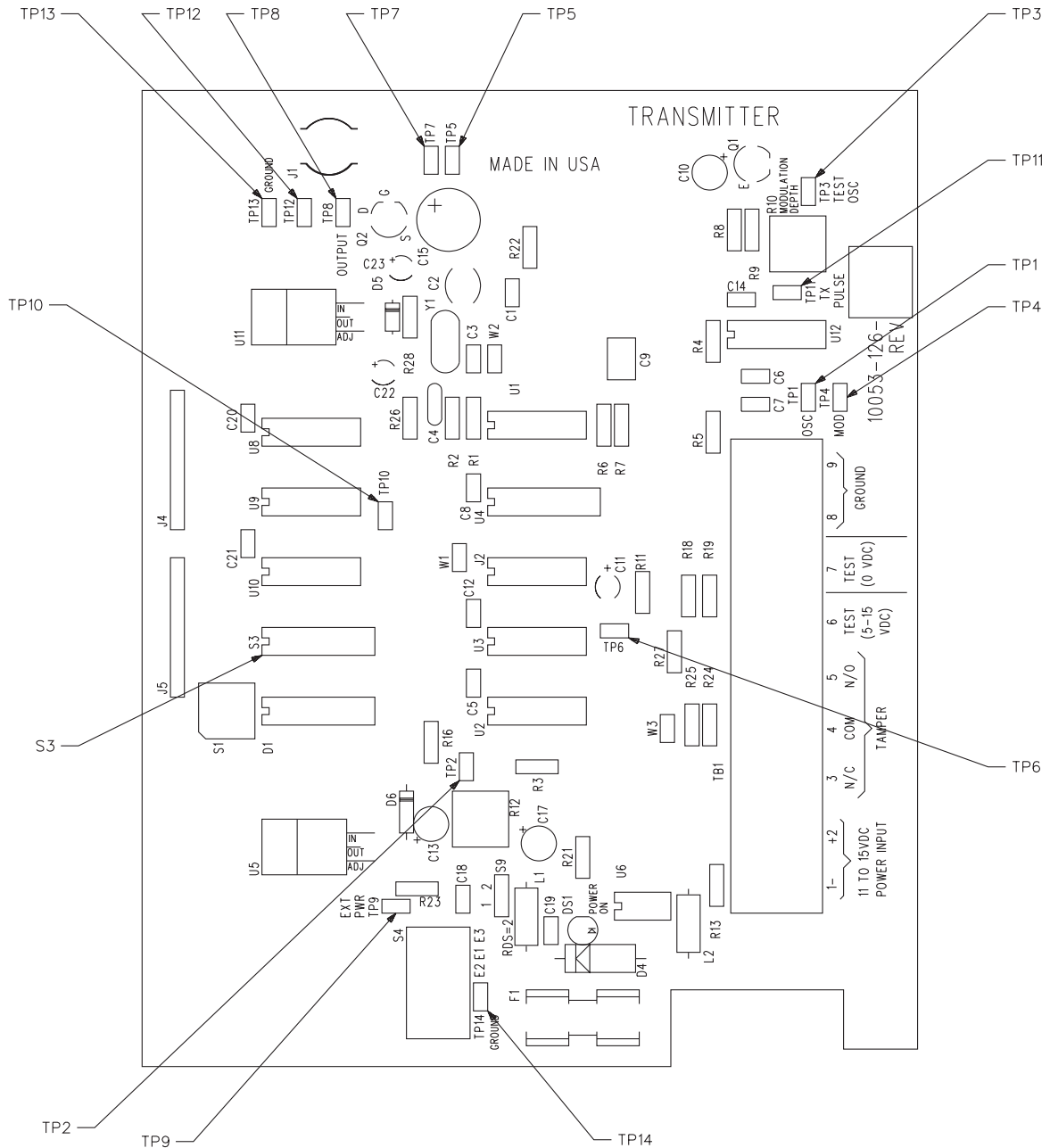
Figure 16. Transmitter Circuit Board Component Location
