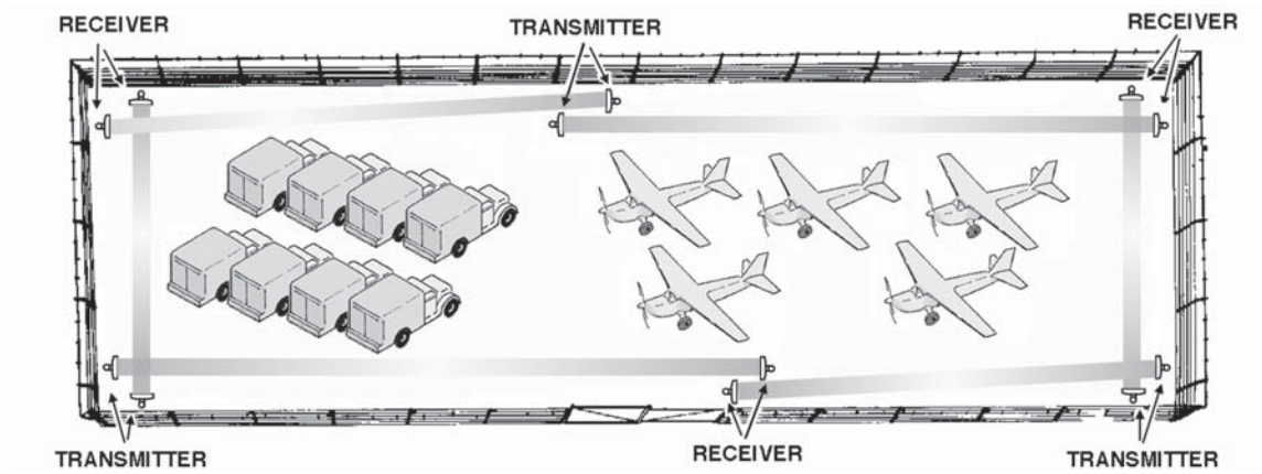
Figure 6. Perimeter Layout
