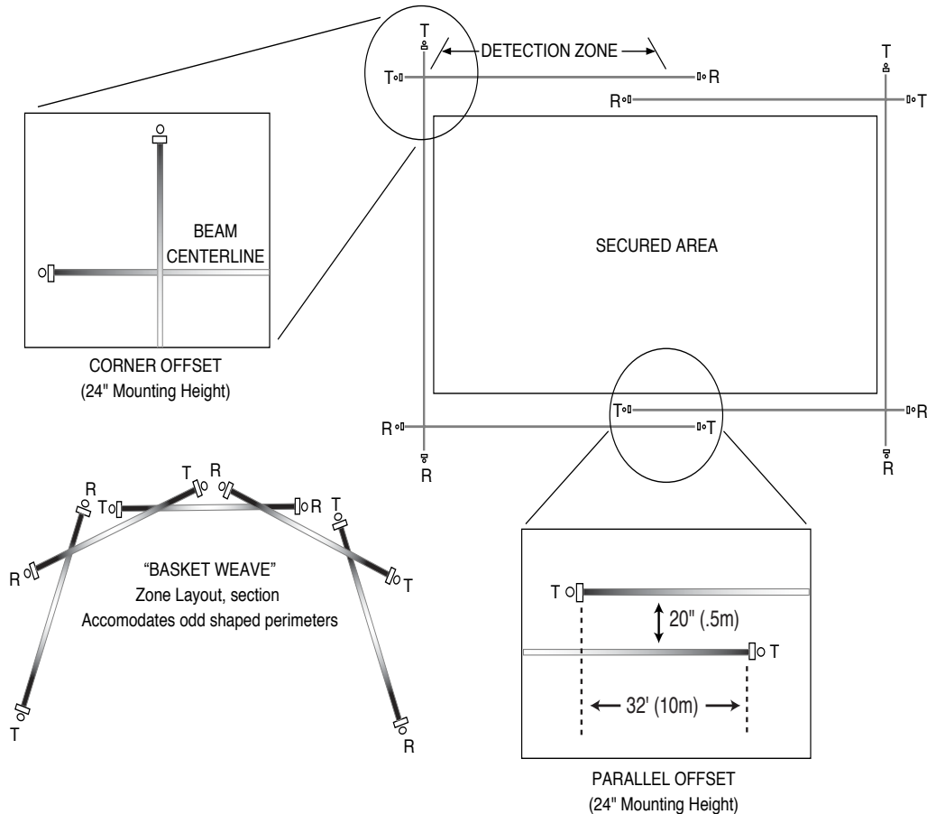
Figure 8. Offset Arrangements: Typical High Security Installation
