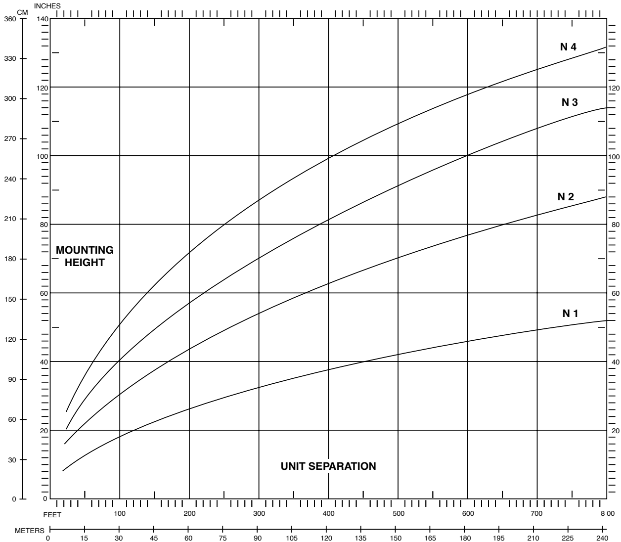
Figure 10. Mounting Height Chart
