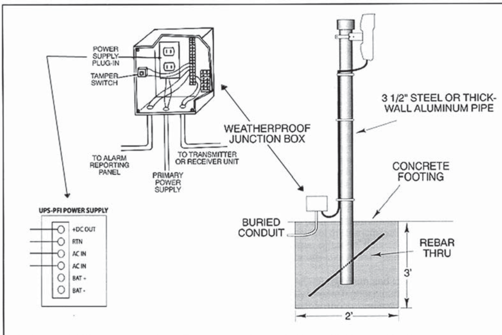
Figure 9. Post Installation & Mounting Units
